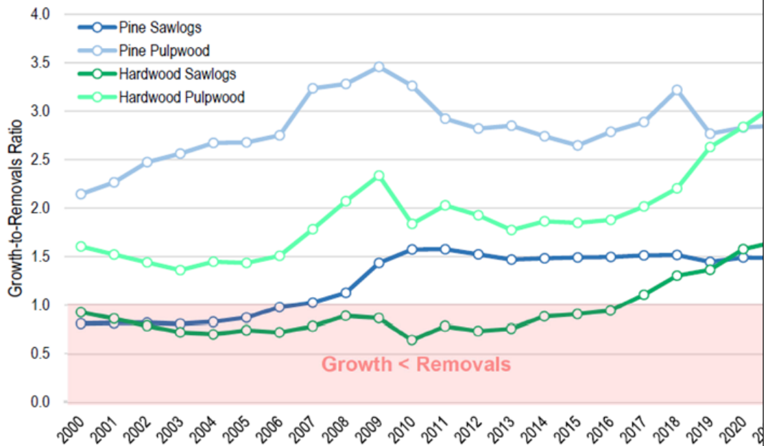
Figure 26. Alabama Cluster Catchment Area – Growth-to-Removals Ratios by Major Timber Product (2000-2020)
