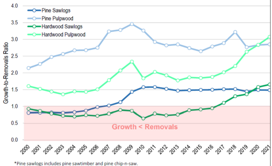
Figure 26. Alabama Cluster Catchment Area – Growth-to-Removals Ratios by Major Timber Product (2000-2021)
