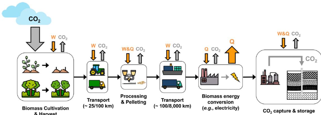
Figure 4: The life cycle of BECCS. Biomass is usually transported via road to where, if necessary, it is processed into pellets before being shipped to the power generation and storage facilities. Grey arrows show uptake and leakage of CO 2 over the entire life cycle, orange arrows show energy consumption and production, W is power, Q is heat. Source: Chiquier et al. 2022
